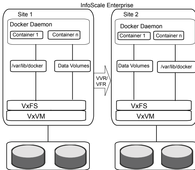
Figure 16-4 Disaster recovery with VVR and VFR technologies
