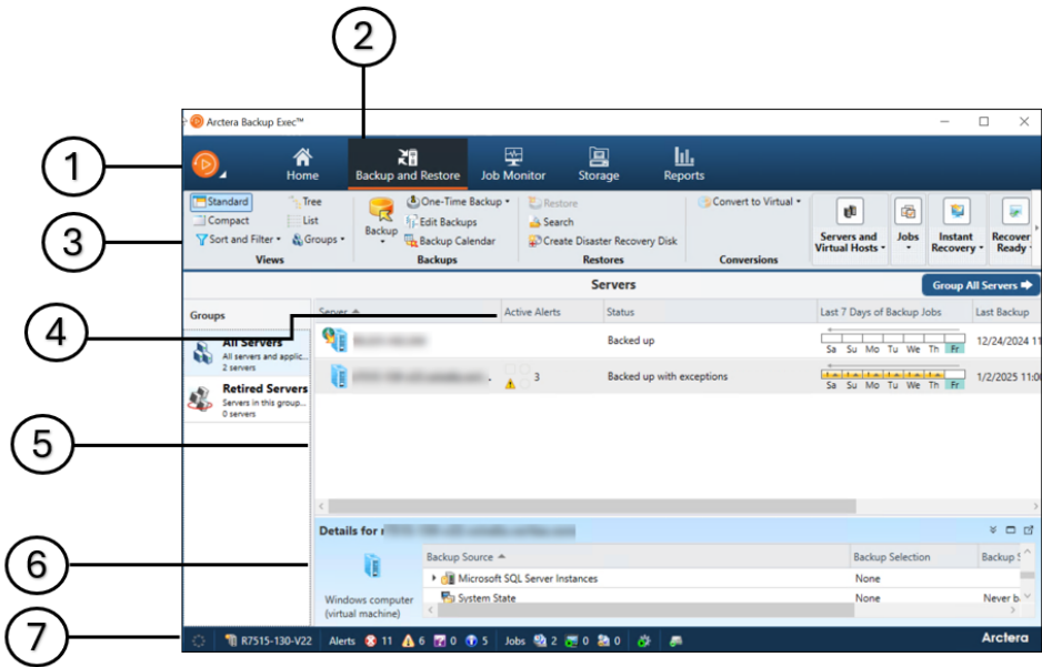
Figure 3-1 Backup Exec Administration Console
