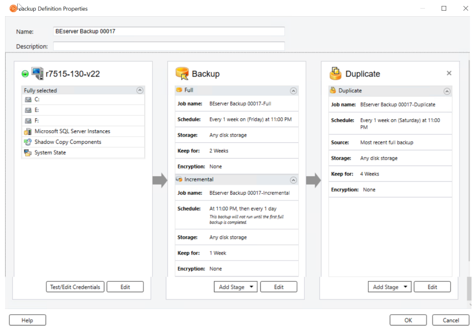
Figure 4-1 Backup Definition (with backup selections, full and incremental backup job templates, and a duplicate stage)
