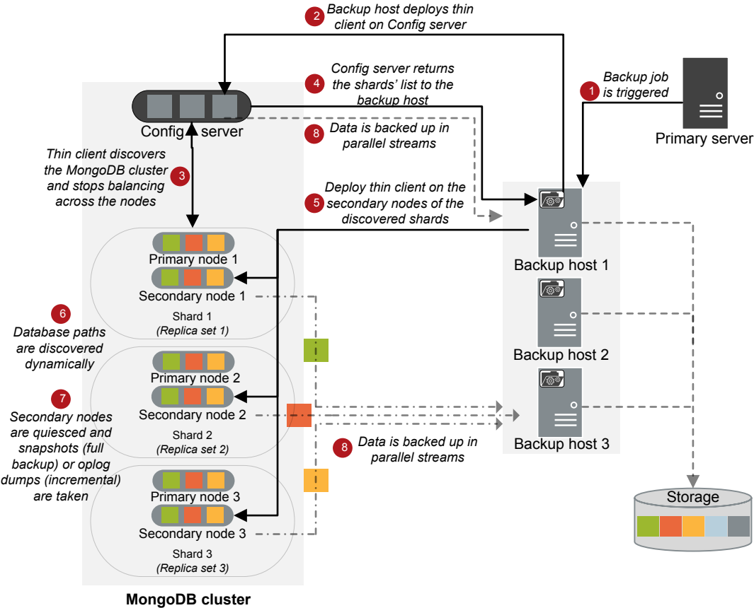
Figure 4-1 Backup flow
