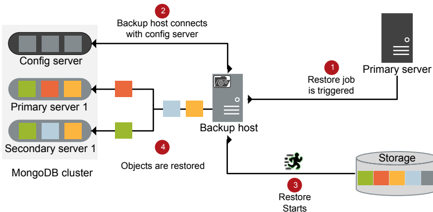
Figure 5-1 Restore flow
