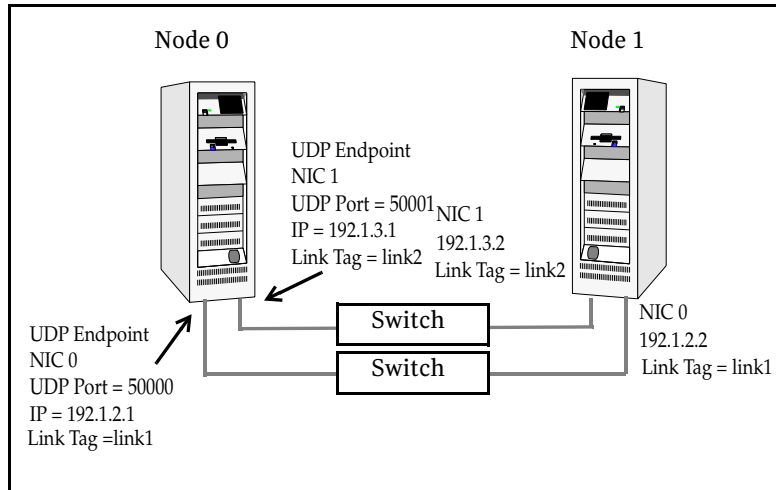
Figure F-1 Direct-attached links employing LLT over UDP
