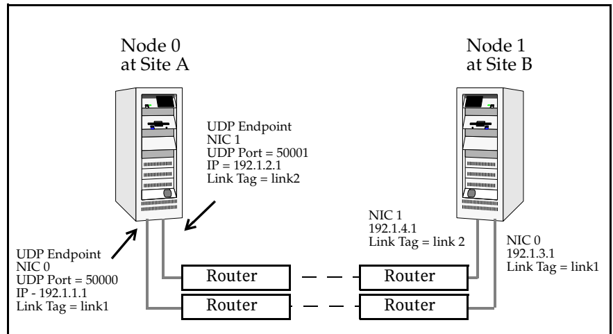
Figure F-2 Links crossing an IP router employing LLT over UDP
