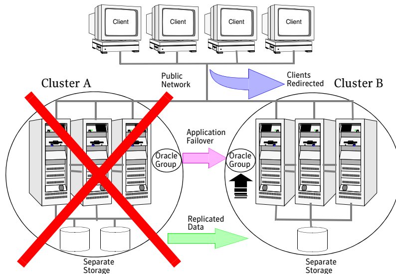
Figure 16-1 Sample global cluster setup
