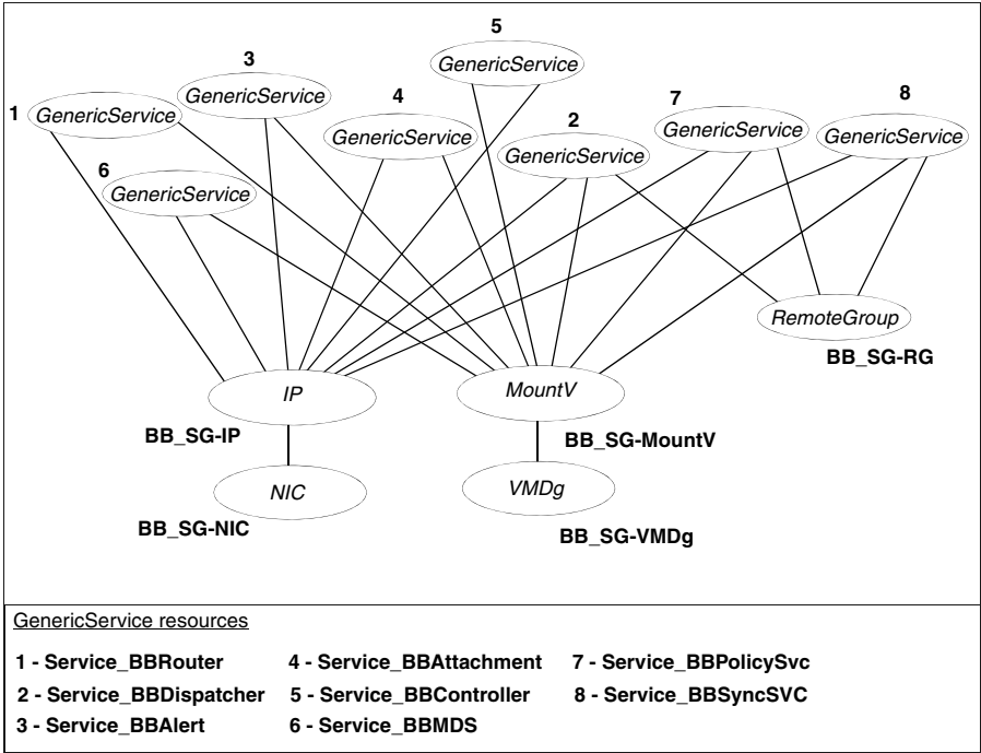
Figure 9-1 BlackBerry Enterprise Server service group dependency graph
