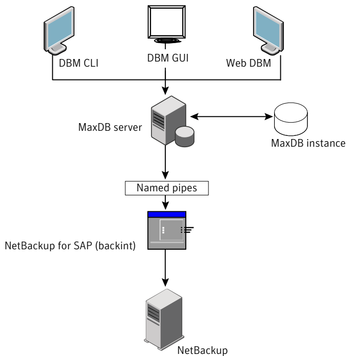
Figure 1-5 Software components for a NetBackup for SAP on MaxDB database environment
