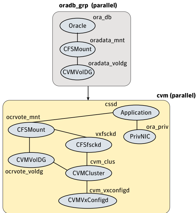
Figure C-1 Service group configuration for sfrac01_main.cf file
