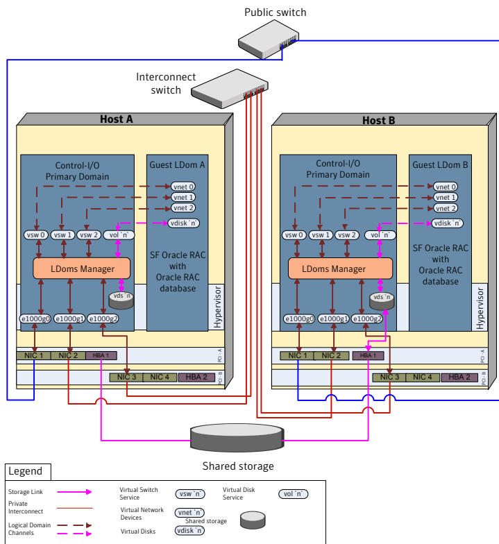
Figure H-12 SF Oracle RAC with Oracle RAC database on guest domains of two hosts
