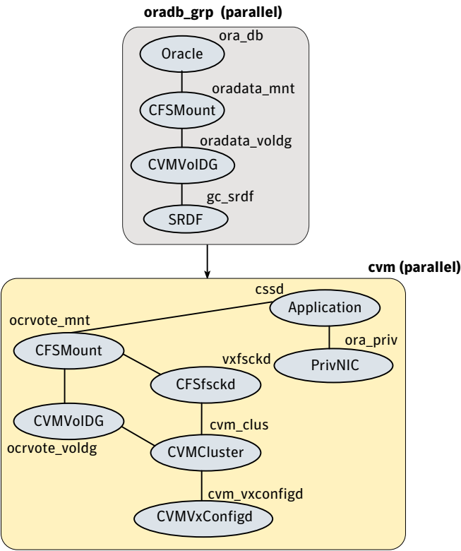
Figure C-8 Service group configuration for sfrac09_main.cf file
