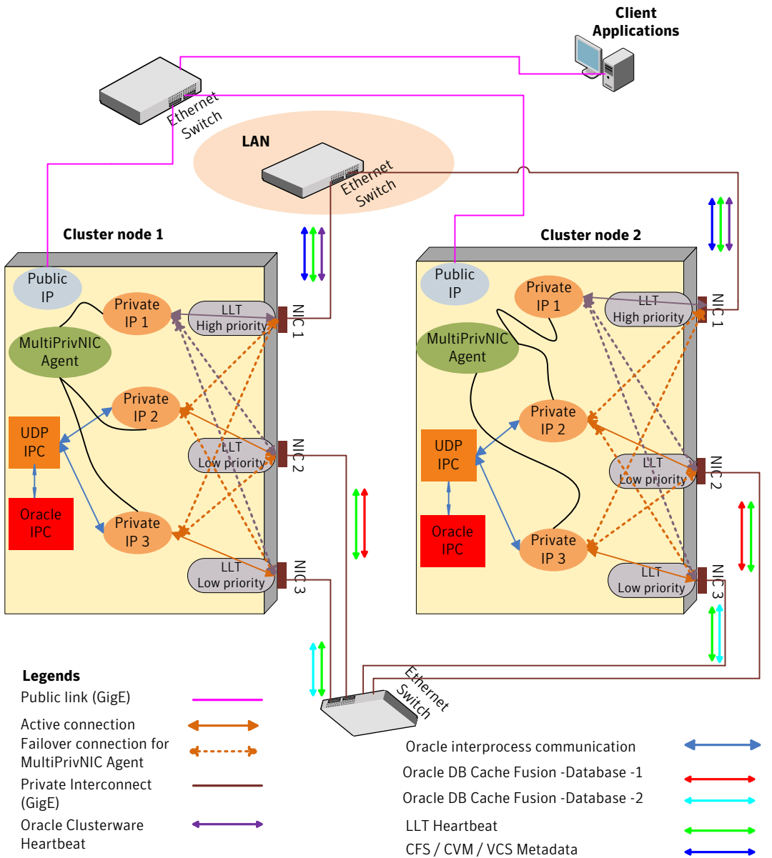
Figure H-4 SF Oracle RAC cluster with isolated Oracle traffic and MultiPrivNIC agent
