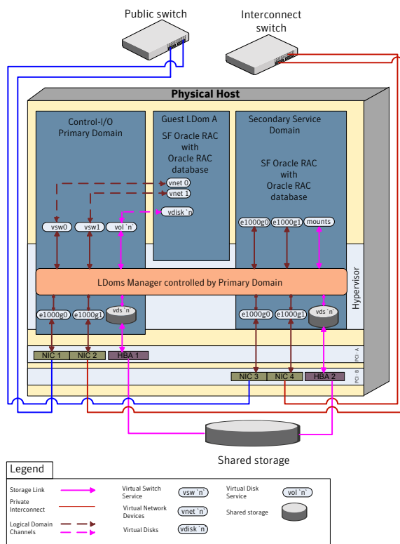
Figure H-14 SF Oracle RAC with Oracle RAC database on I/O domain and guest domain of single host
