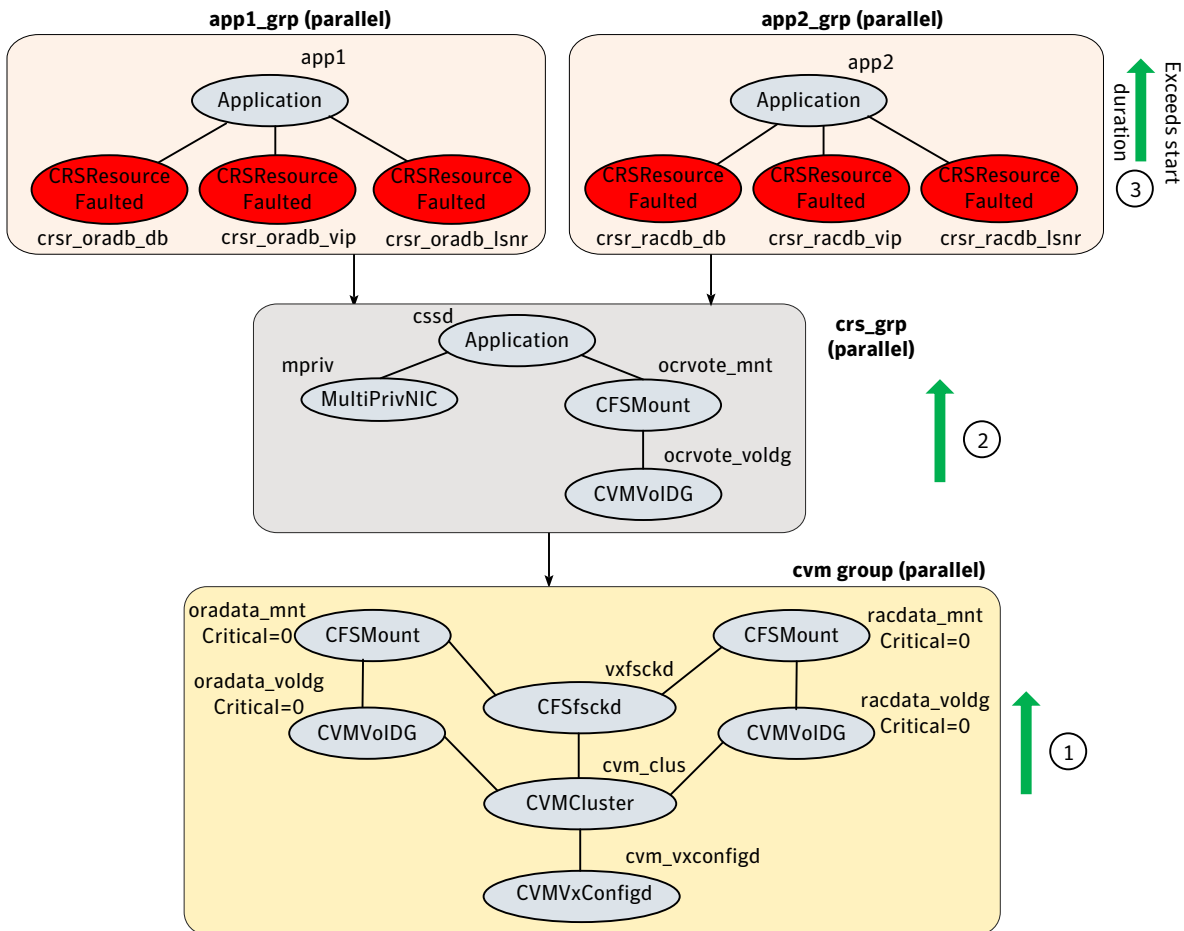
Figure G-6 CRSResource fault at system startup
