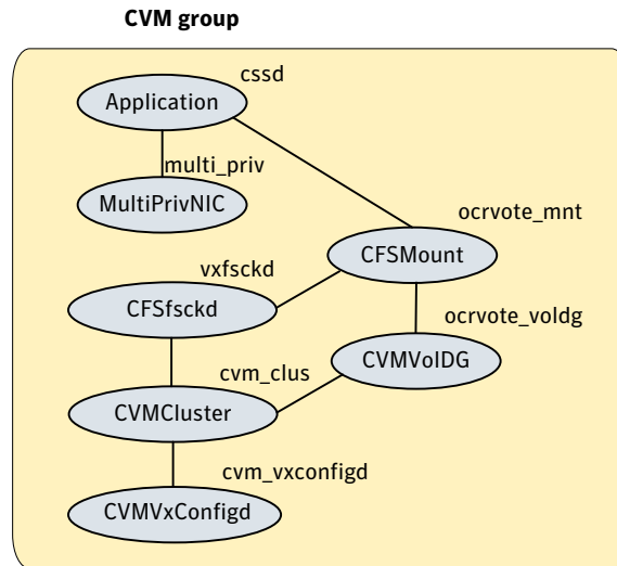
Figure 21-3 Service group configuration without VCS Oracle agent (single database)
