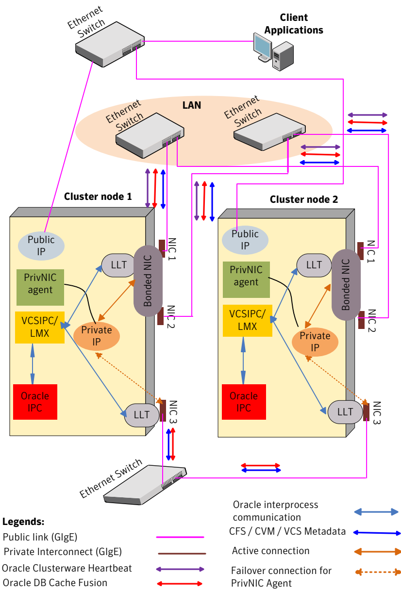
Figure H-5 SF Oracle RAC cluster with NIC bonding, VCS IPC and PrivNIC agent (Oracle RAC 10g)
