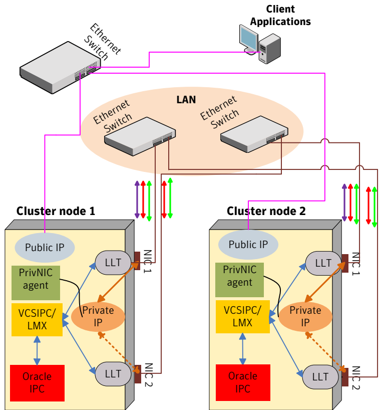
Figure H-1 SF Oracle RAC cluster with VCS IPC and PrivNIC agent (Oracle RAC 10g)
