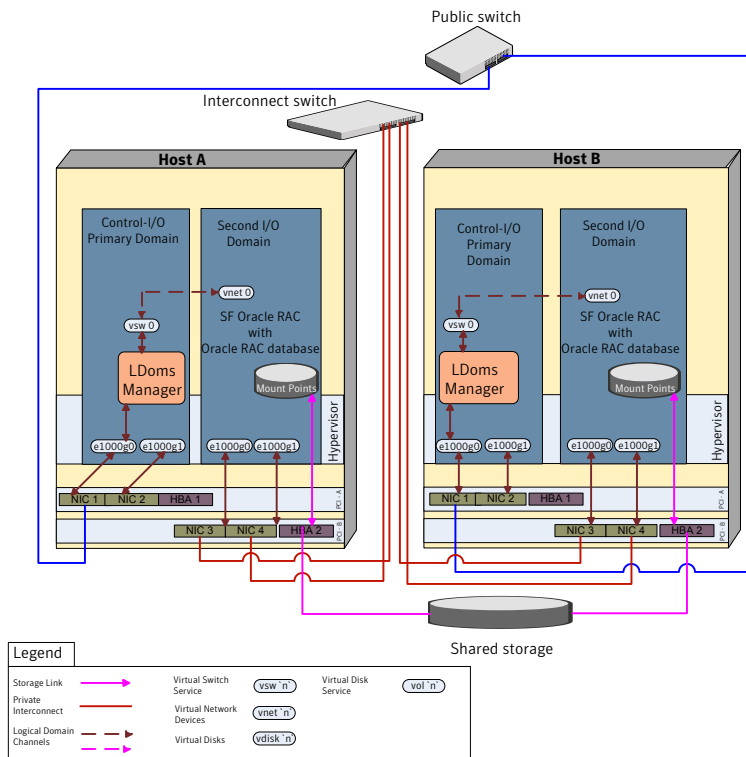
Figure H-11 SF Oracle RAC with Oracle RAC database on I/O domains of two hosts
