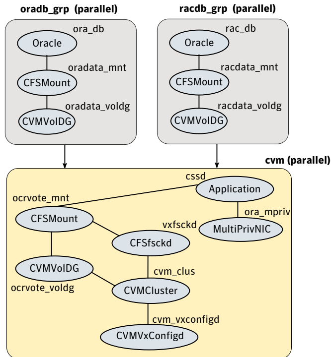
Figure C-3 Service group configuration for sfrac03_main.cf file
