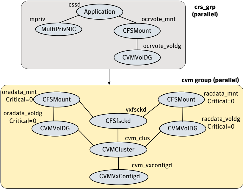
Figure 21-4 Service group configuration without the VCS Oracle agent (multiple databases)
