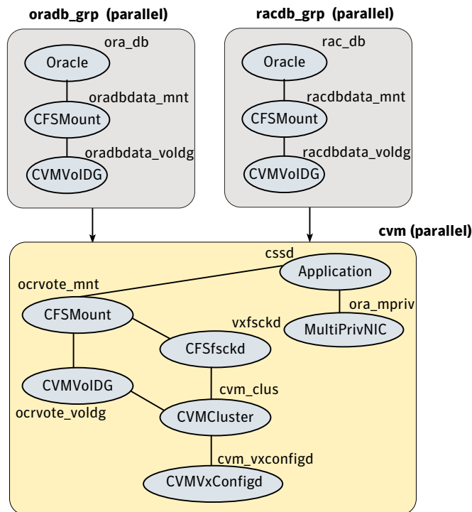
Figure C-6 Service group configuration for sfrac06_main.cf file
