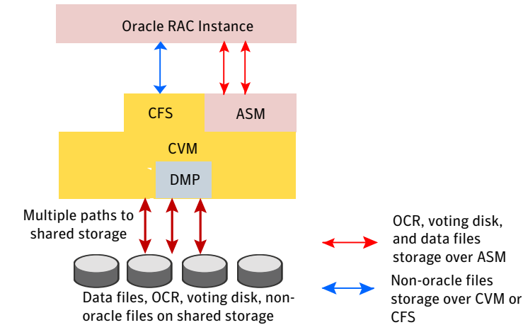
Figure E-3 Supported Oracle RAC configuration (Oracle RAC 11g Release 2)
