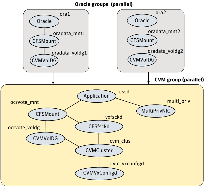
Figure 21-2 Service group configuration with the VCS Oracle agent
