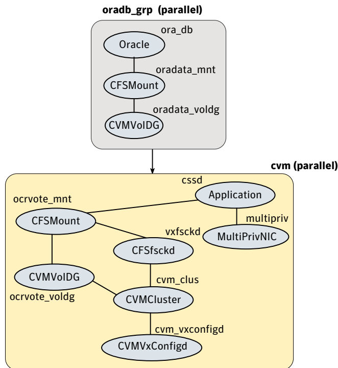
Figure C-10 Service group configuration for sfrac11_main.cf file
