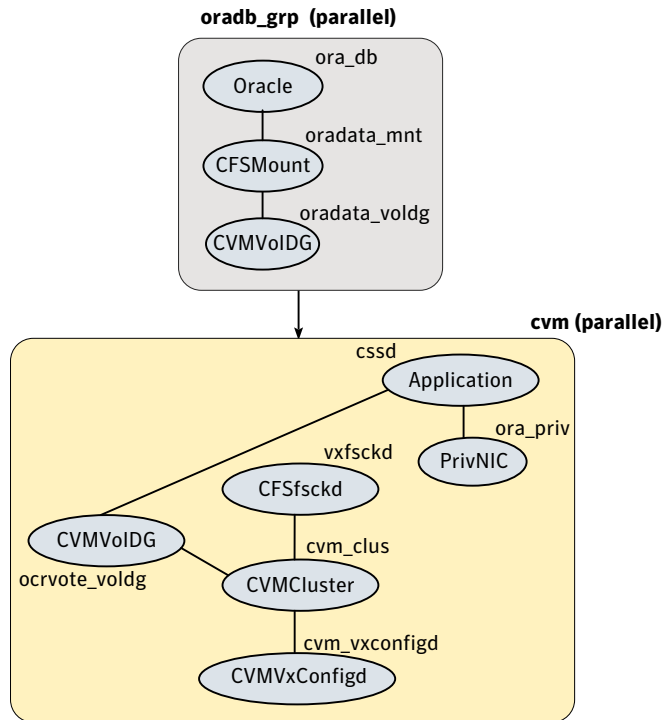
Figure C-2 Service group configuration for sfrac02_main.cf file
