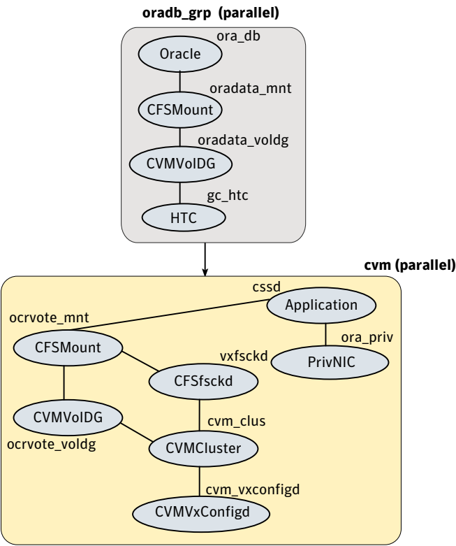
Figure C-11 Service group configuration for sfrac12_main.cf file
