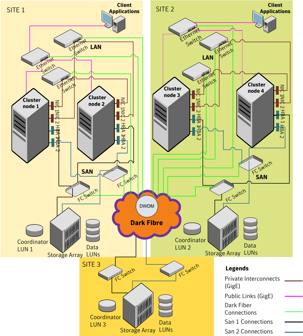
Figure 1-5 Basic campus cluster setup
