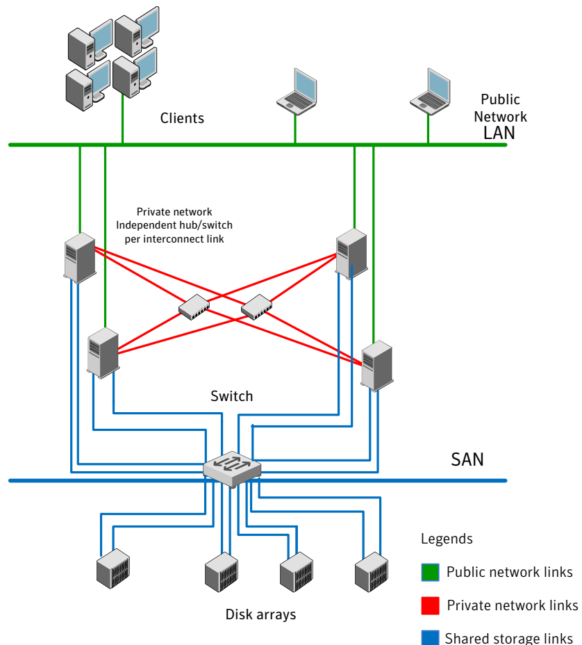
Figure 1-2 Sample four-node SF Oracle RAC cluster
