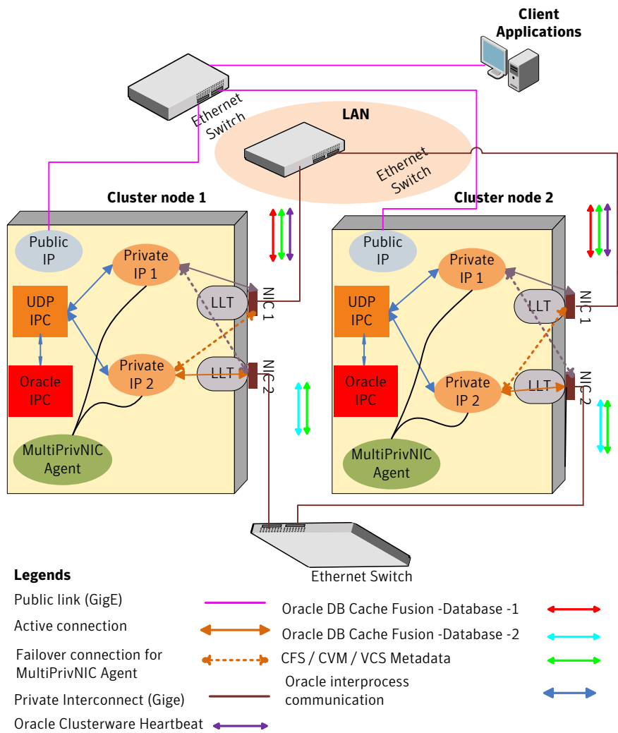
Figure H-3 SF Oracle RAC cluster for multiple databases with UDP IPC and MultiPrivNIC agent
