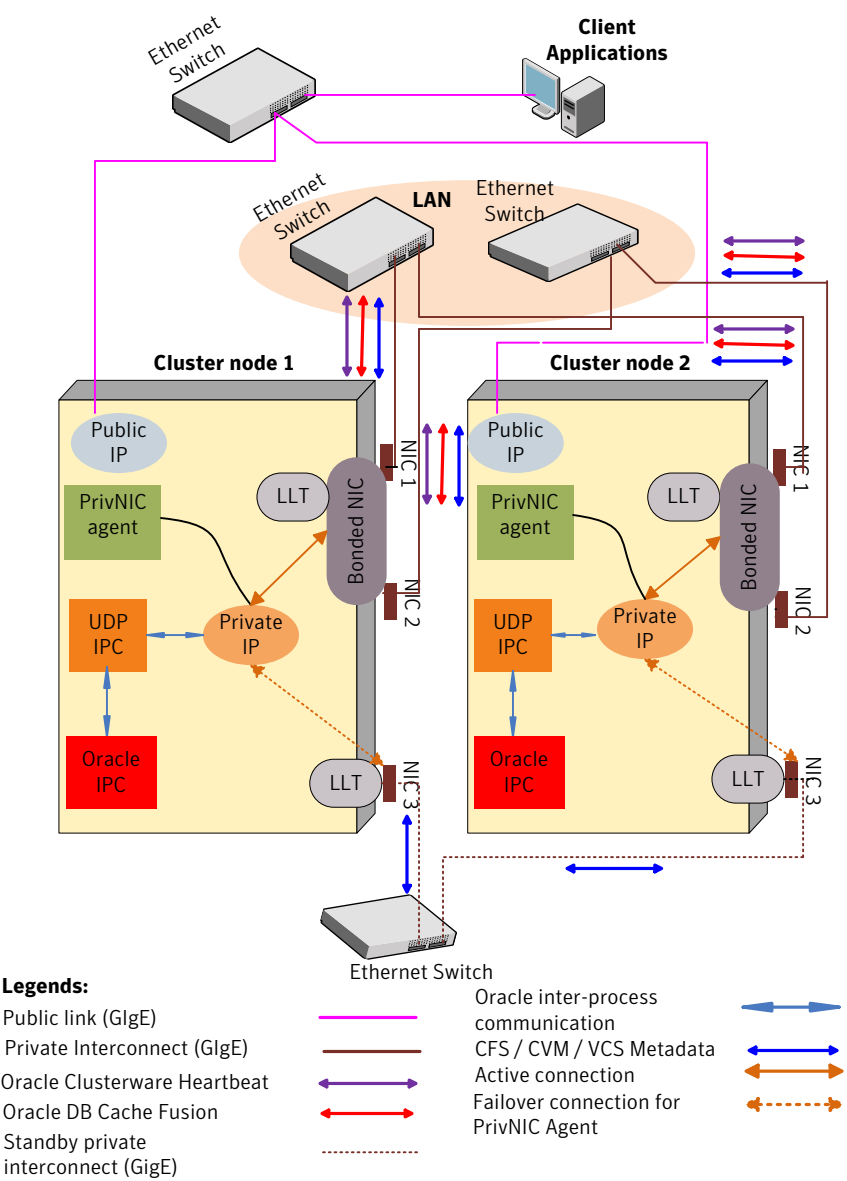
Figure H-6 SF Oracle RAC cluster with NIC bonding, UDP IPC, and PrivNIC agent
