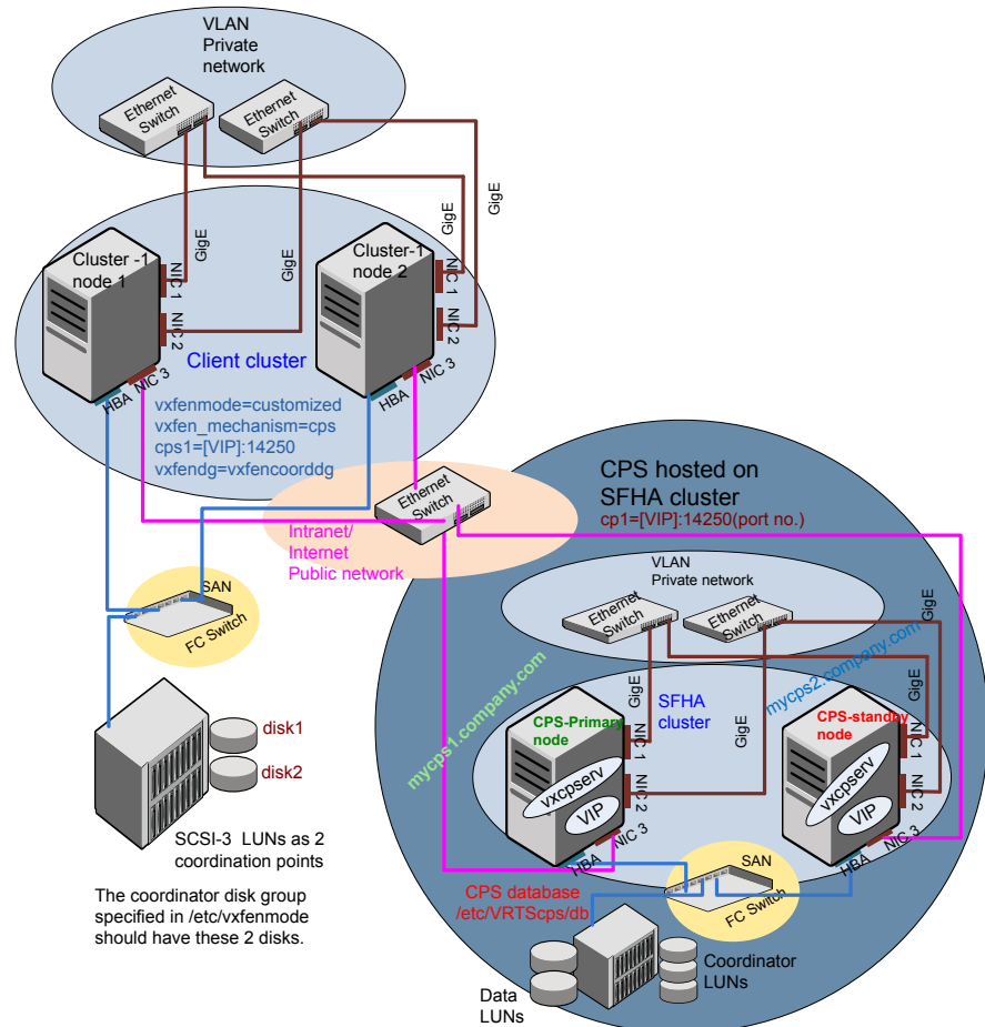
Figure H-8 Client cluster served by highly available CP server and 2 SCSI-3 disks
