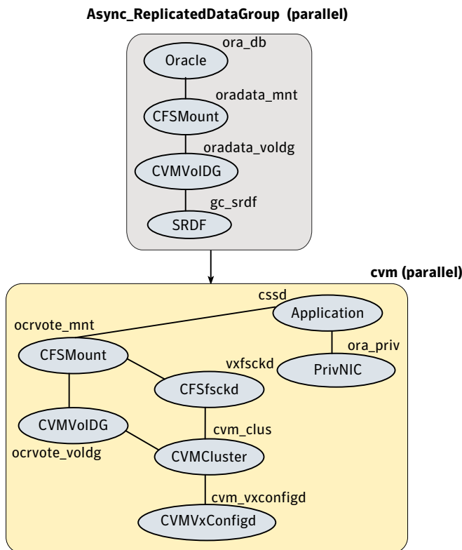
Figure C-9 Service group configuration for sfrac10_main.cf file
