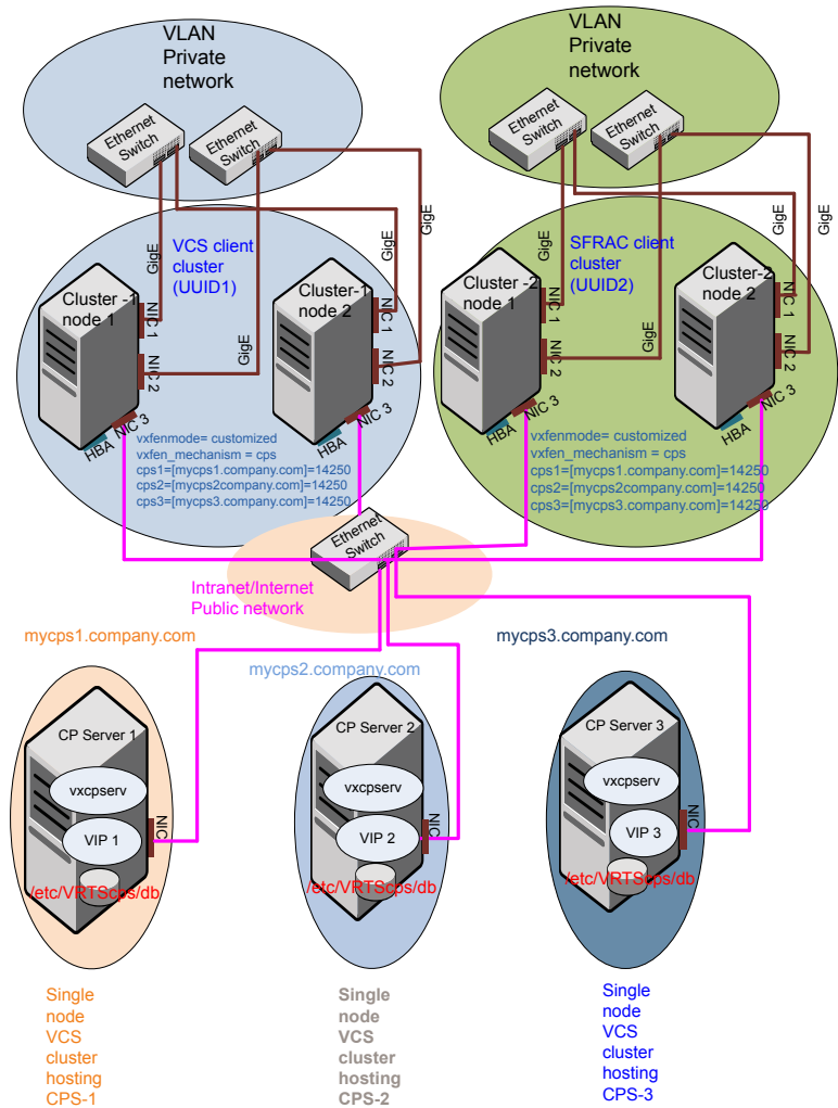
Figure H-7 Two unique client clusters served by 3 CP servers
