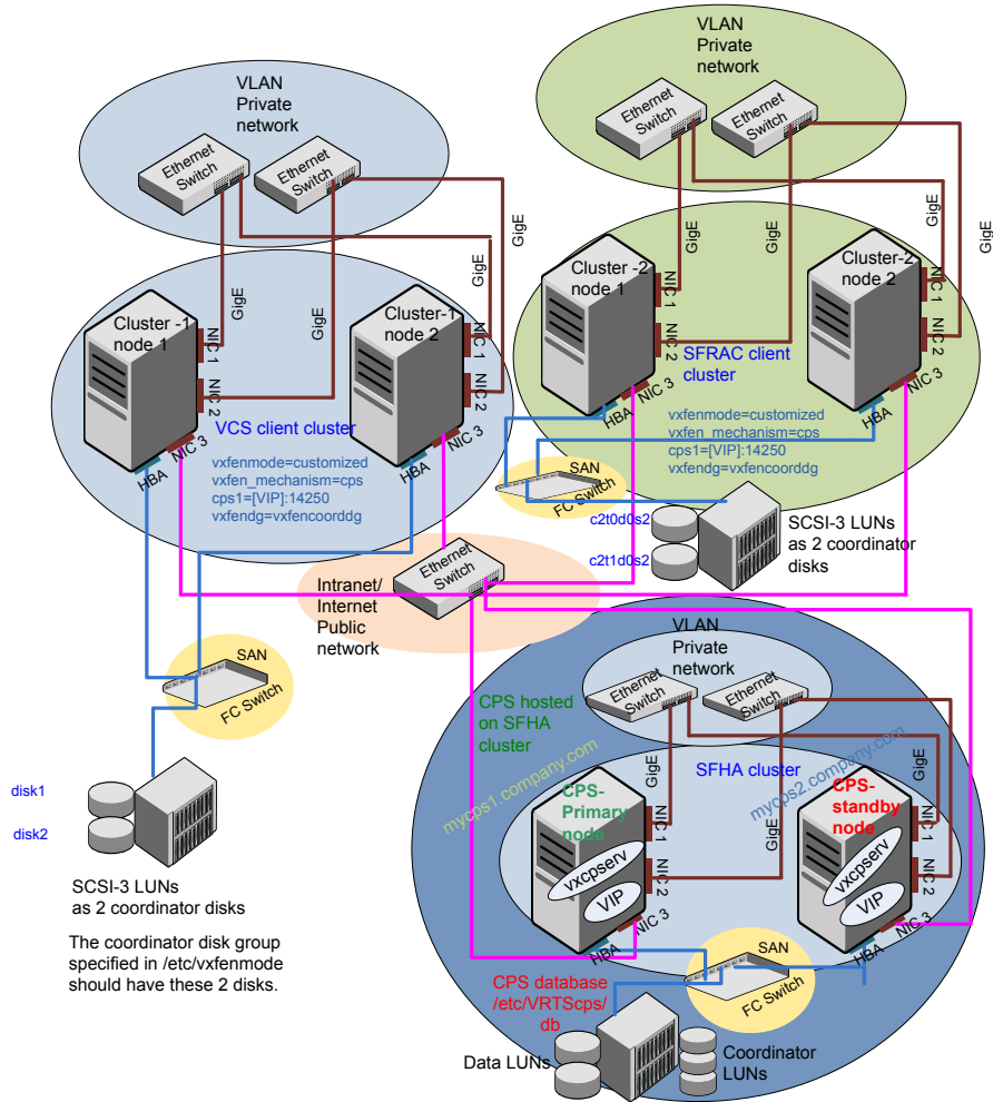
Figure H-10 Multiple client clusters served by highly available CP server and 2 SCSI-3 disks
