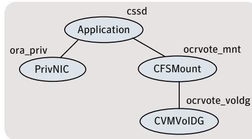
Figure G-1 Basic service group configuration with the PrivNIC agent
