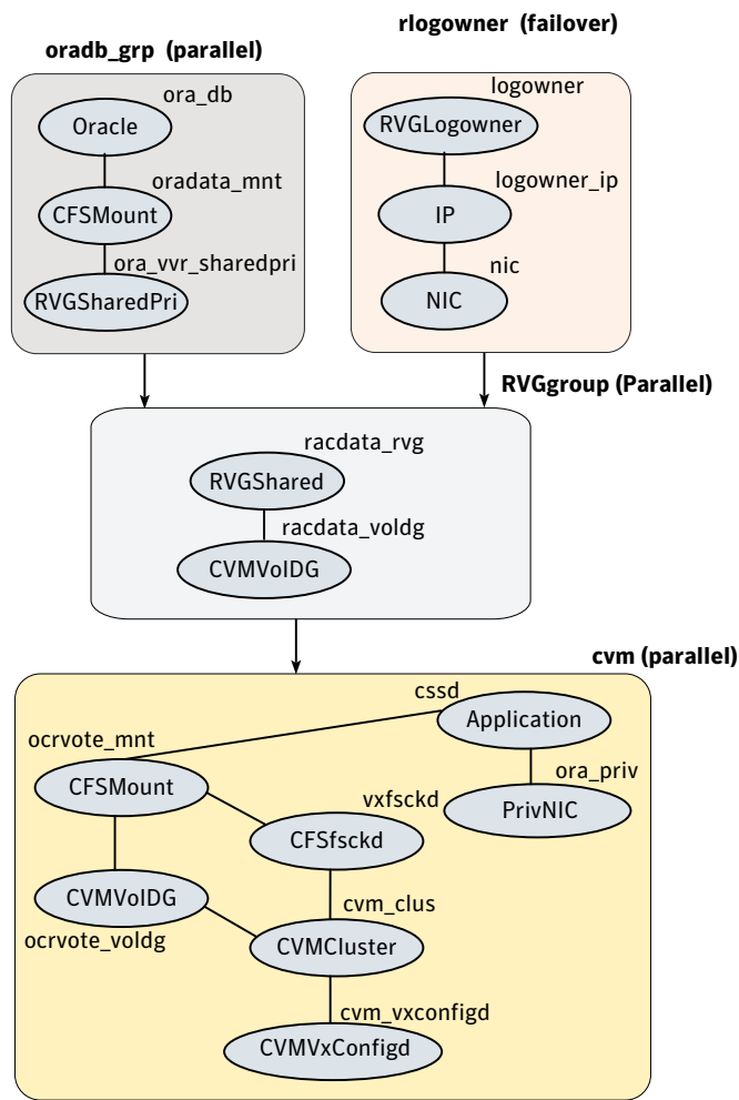
Figure C-7 Service group configuration for sfrac07_main.cf and sfrac08_main.cf files
