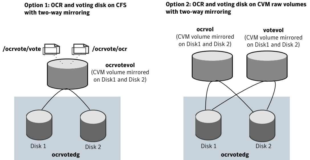
Figure 3-1 OCR and voting disk storage options
