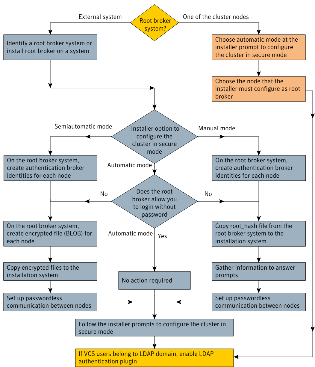
Figure 7-1 Workflow to configure SF Oracle RAC cluster in secure mode
