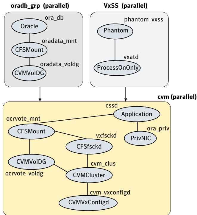
Figure C-13 Service group configuration for sfrac14_main.cf file
