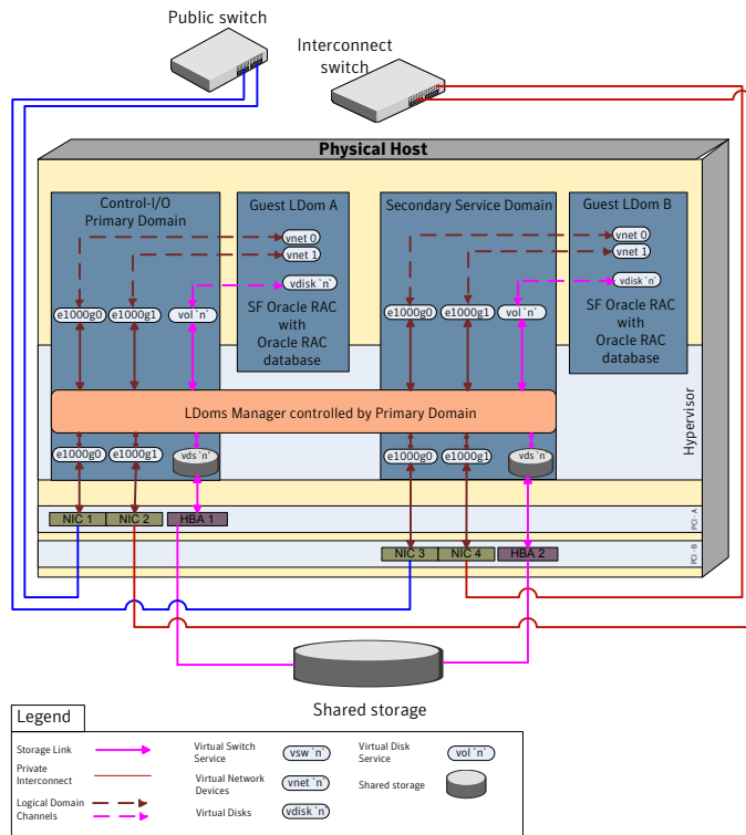
Figure H-13 SF Oracle RAC with Oracle RAC database on guest domains of single host
