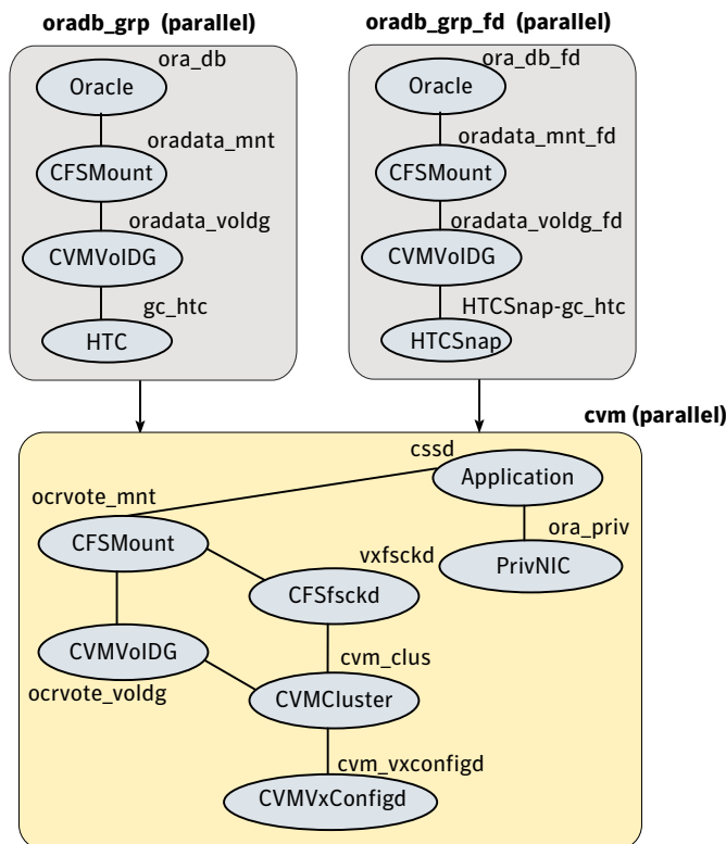
Figure C-12 Service group configuration for sfrac13_main.cf file
