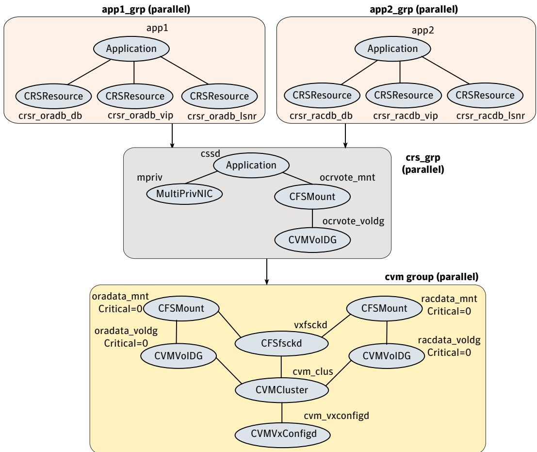
Figure C-4 Service group configuration for sfrac04_main.cf file
