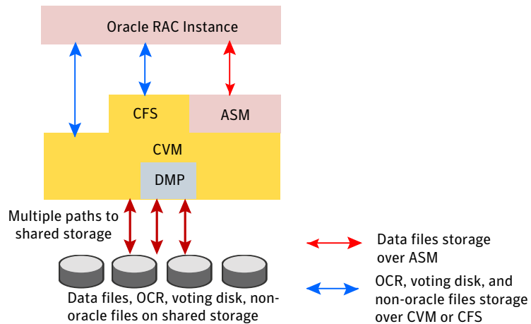
Figure E-2 Supported Oracle RAC configuration (all supported Oracle RAC versions)
