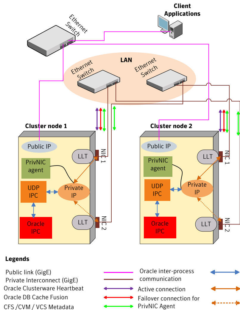
Figure H-2 SF Oracle RAC cluster with UDP IPC and PrivNIC agent
