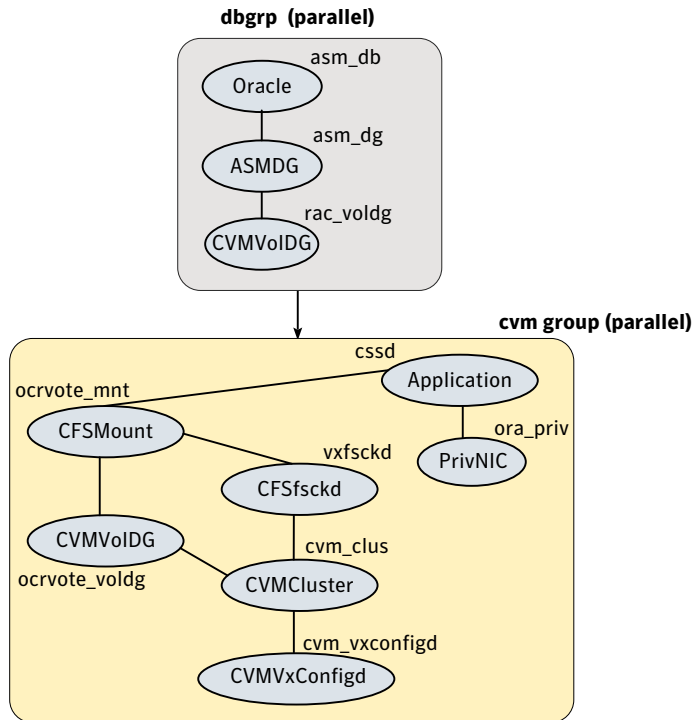
Figure C-5 Service group configuration for sfrac05_main.cf file
