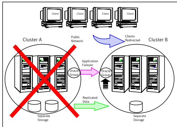
Figure 1-6 Global clusters
