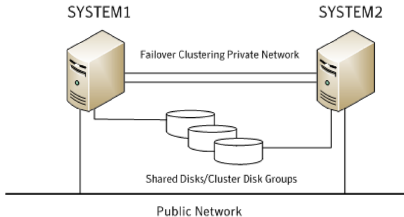
Figure 1-1 High availability active/passive configuration
