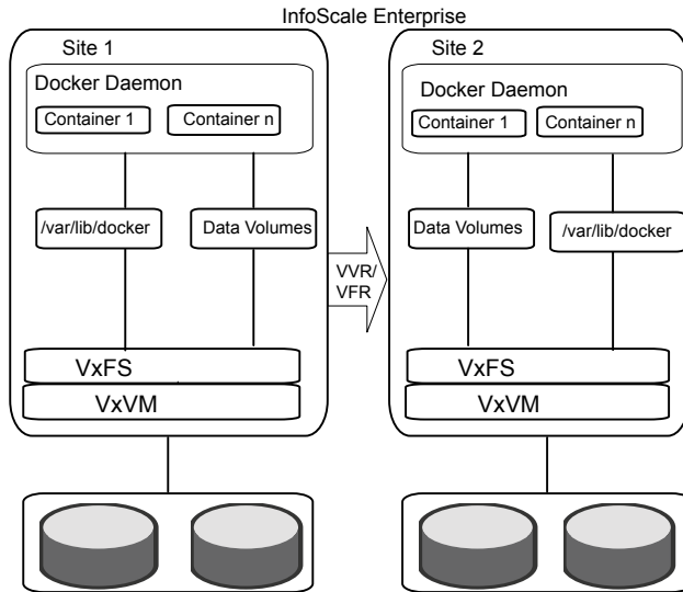
Figure 20-4 Disaster recovery with VVR and VFR technologies
