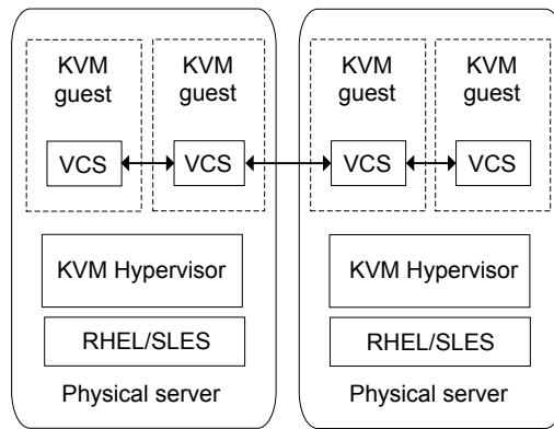
Figure 2-9 Cluster Server in the guest
