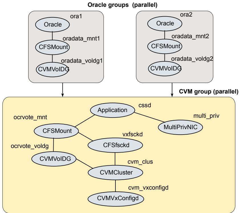
Figure 15-2 illustrates a service group configuration for container and pluggable databases with the VCS Oracle agent.
