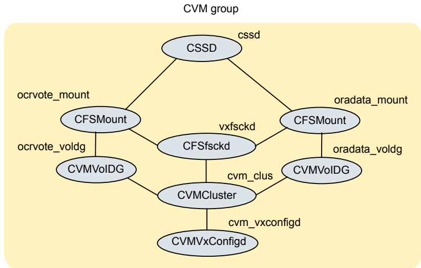
Figure 15-6 illustrates a sample service group configuration in the absence of the VCS Oracle agent for multiple database configurations.
