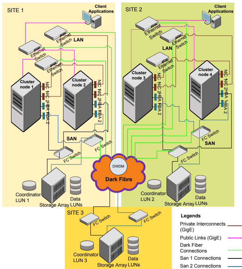
Figure 19-1 Sample SF Oracle RAC configuration
