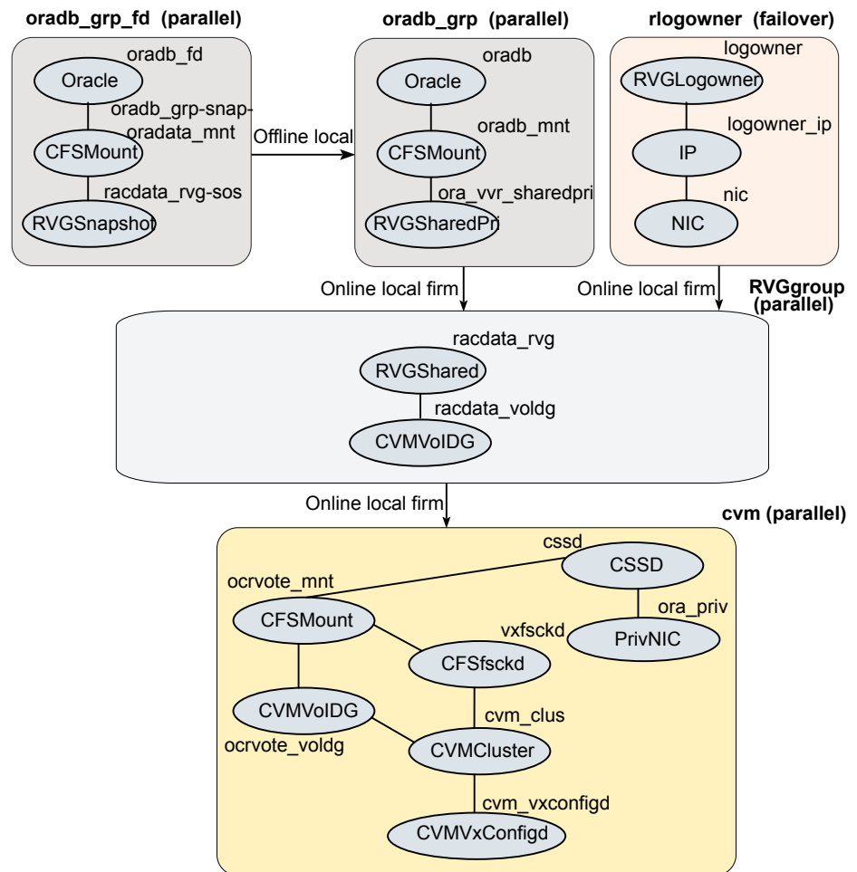
Figure 2-1 Service group configuration for fire drill
