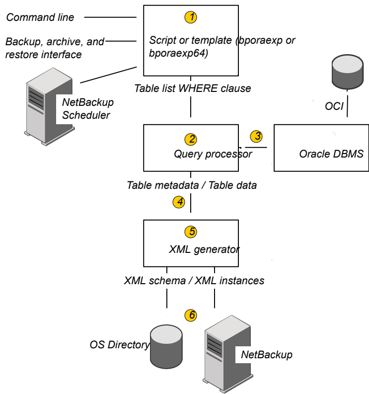
Figure G-1 XML export archives
