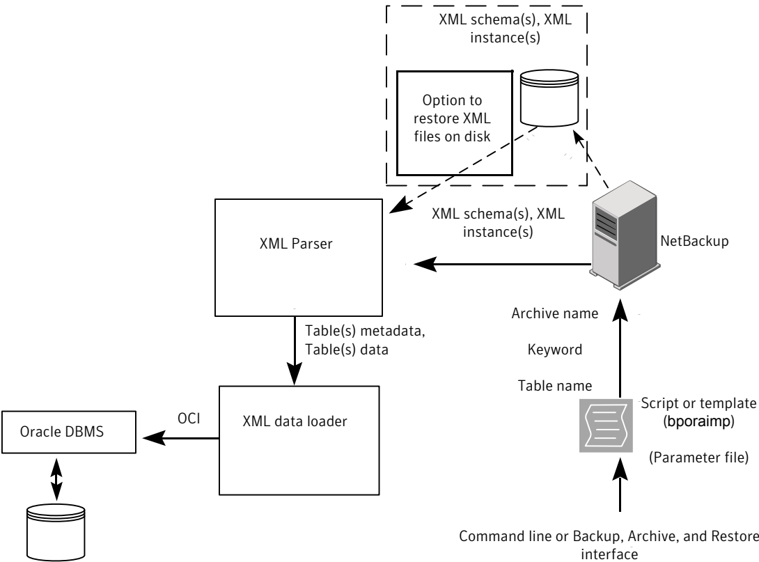
Figure G-4 XML import restore data flow
