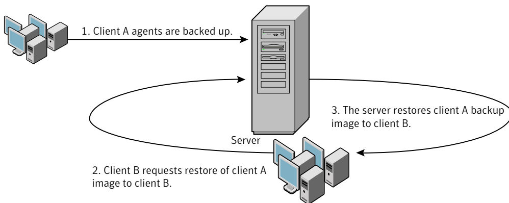
Figure 5-1 Redirected restore
