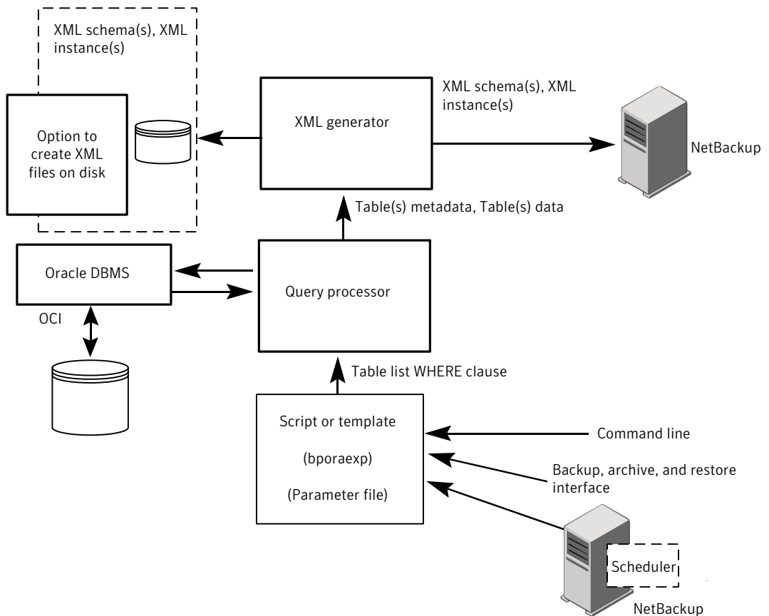
Figure G-2 XML export archive data flow
