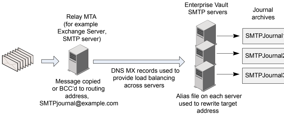
Figure 5-2 SMTP Journaling with address rewriting
