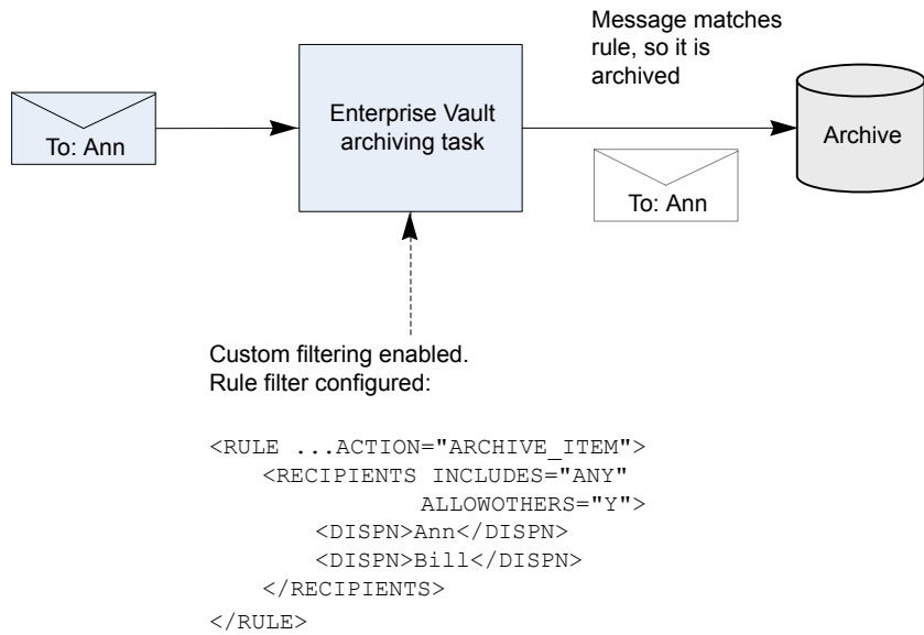
Figure 5-2 Msg 1 with INCLUDES="ANY" and ALLOWOTHERS="Y"
