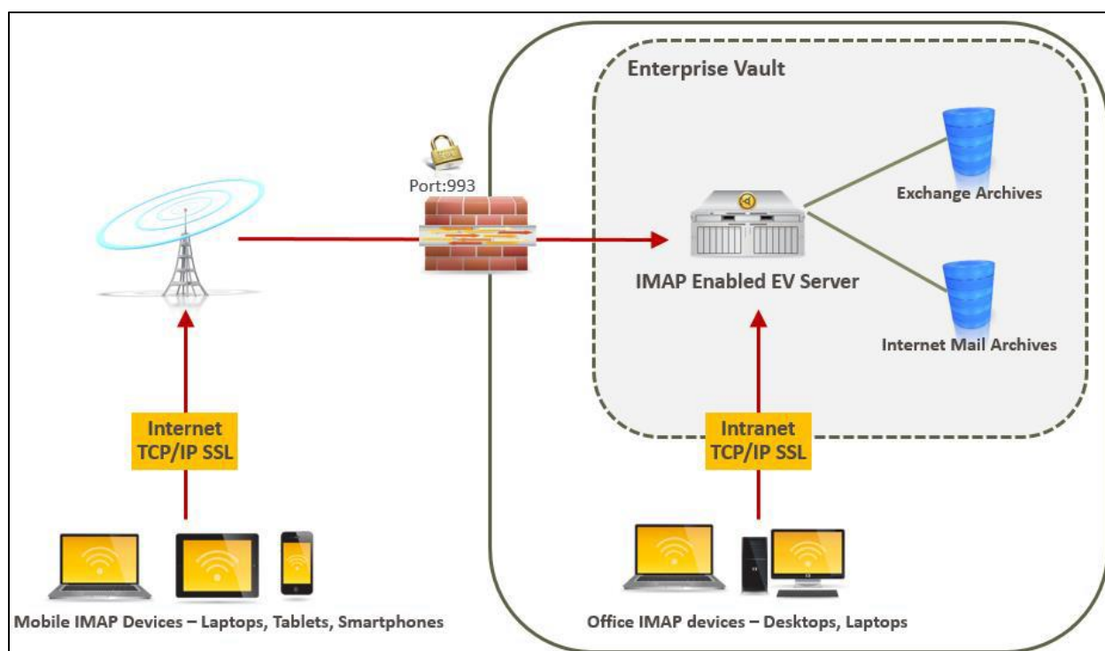
Figure 1 – IMAP Access Architecture Overview
