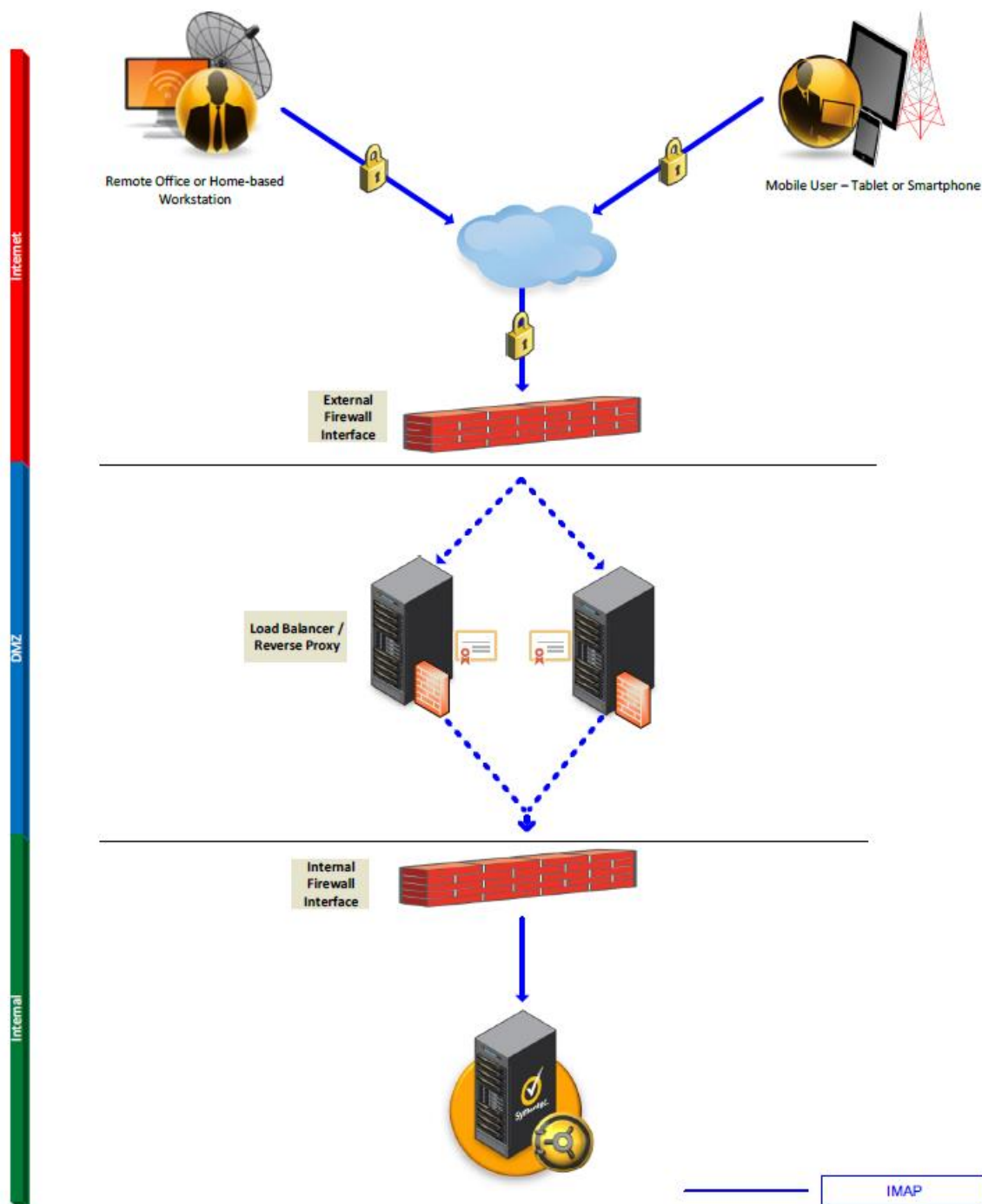
Figure 7 – Example IMAP configuration for External/Internet Clients
