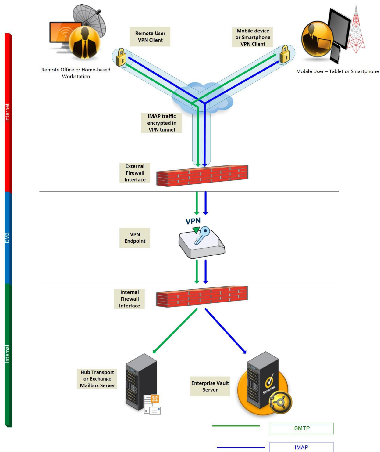
Figure 5 – Remote IMAP access using a VPN client
