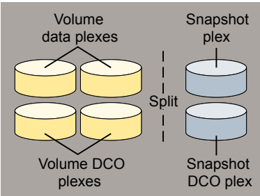
Figure 41-4 Examples of disk groups that can and cannot be split
