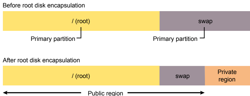
Figure 32-2 Root and swap configured on two primary partitions, and no free space
