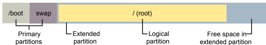
Figure 32-9 Workaround by growing the extended partition
