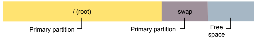
Figure 32-1 Root and swap configured on two primary partitions, and free space on the disk
