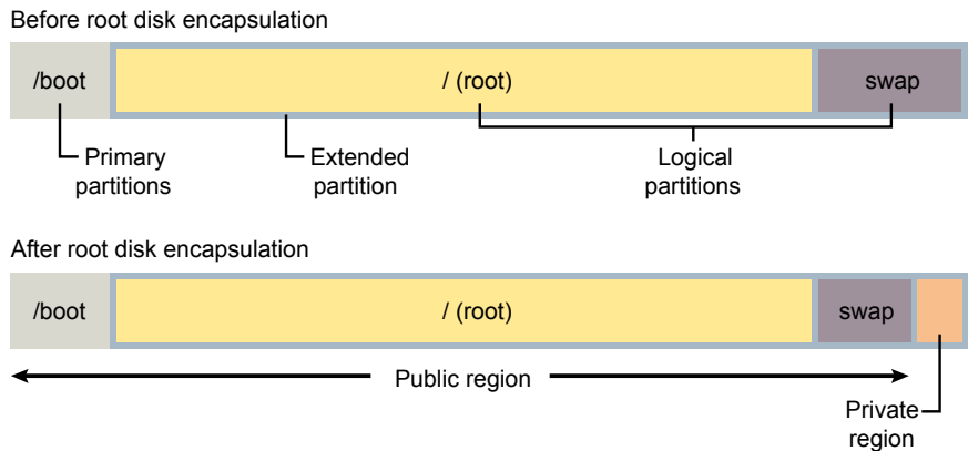
Figure 32-4 Boot configured on a primary partition, and root and swap configured in the extended partition
