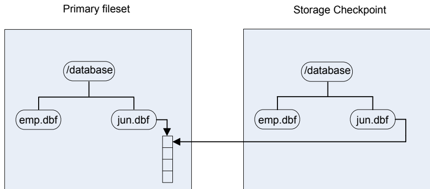
Figure 16-9 Primary fileset and its Storage Checkpoint
