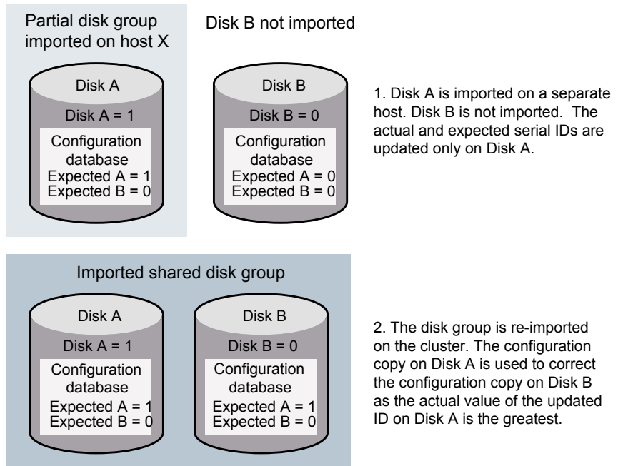
Figure 31-6 Example of a serial split brain condition that can be resolved automatically
