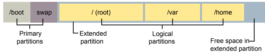
Figure 32-11 Workaround by shrinking existing logical partitions
