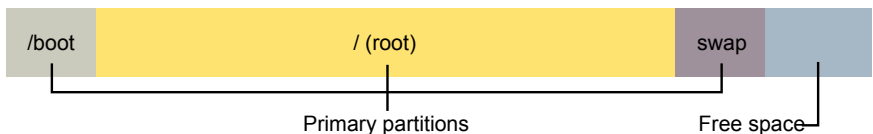
Figure 32-5 Boot, swap and root configured on three primary partitions, and free space on the disk
