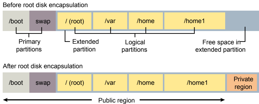
Figure 32-3 Boot and swap configured on two primary partitions, and free space in the extended partition
