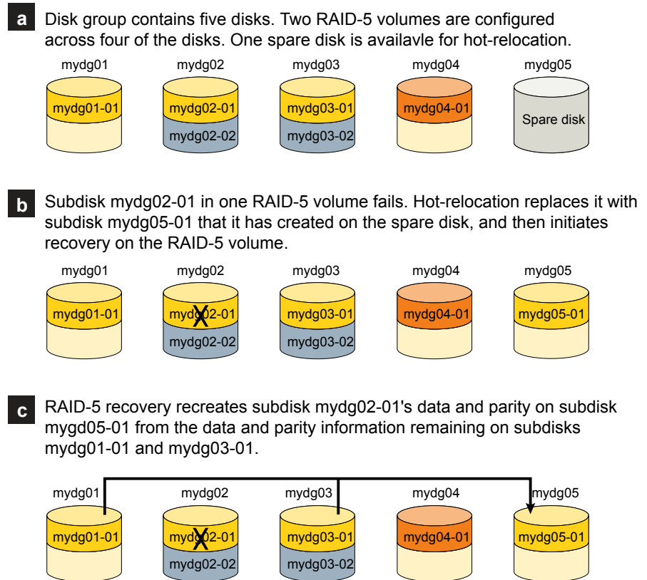
Figure 28-1 Example of hot-relocation for a subdisk in a RAID-5 volume
