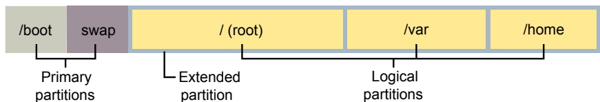
Figure 32-10 Boot and swap configured on two primary partitions, and no free space
