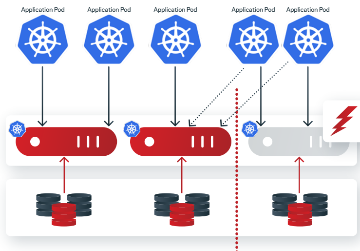
Figure 3. Veritas Alta Shared Storage I/O fencing in Kubernetes helps ensure data integrity
