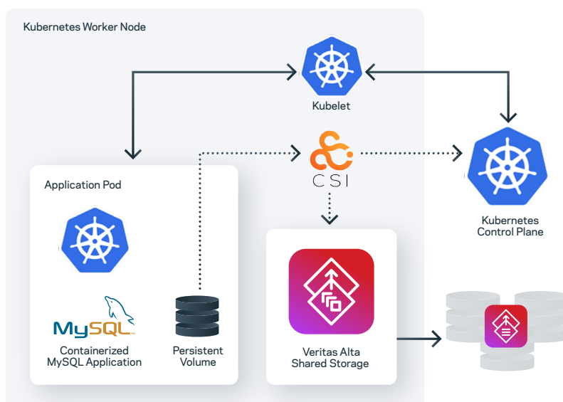
Figure 4. Veritas Alta Shared Storage CSI plug-in overview
