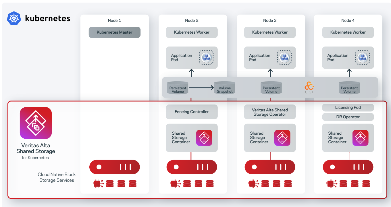
Figure 5. Veritas Alta Shared Storage persistent volumes and persistent volume snapshots
