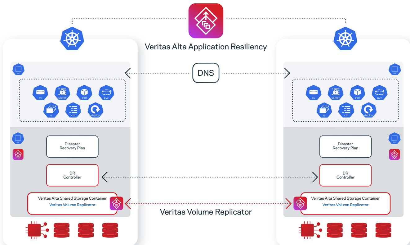
Figure 2. Veritas Alta Application Resiliency DR manager for Kubernetes
