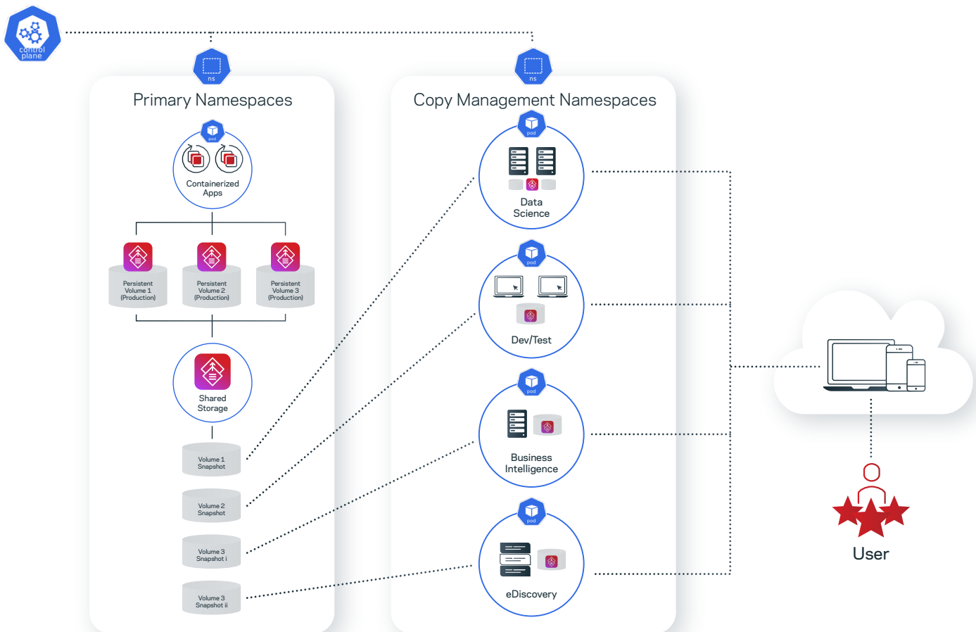
Figure 6. Veritas Alta Storage Resiliency persistent volumes and persistent volume snapshots used for multiple purposes
