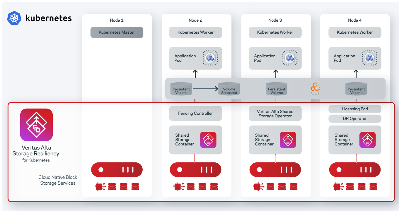
Figure 5. Veritas Alta Storage Resiliency persistent volumes and persistent volume snapshots
