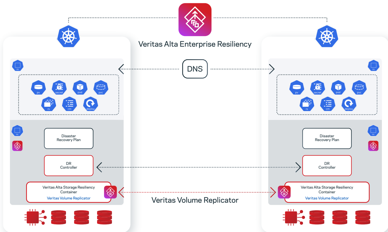
Figure 2. Veritas Alta Enterprise Resiliency DR manager for Kubernetes
