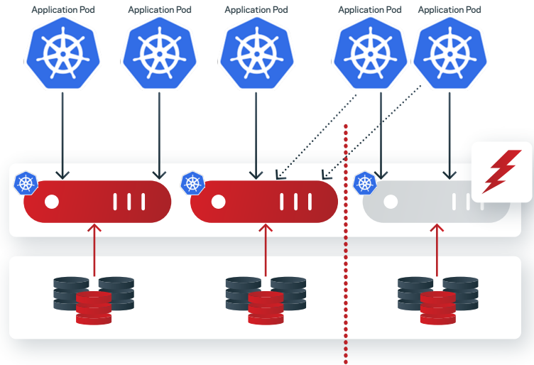
Figure 3. Veritas Alta Storage Resiliency I/O fencing in Kubernetes helps ensure data integrity
