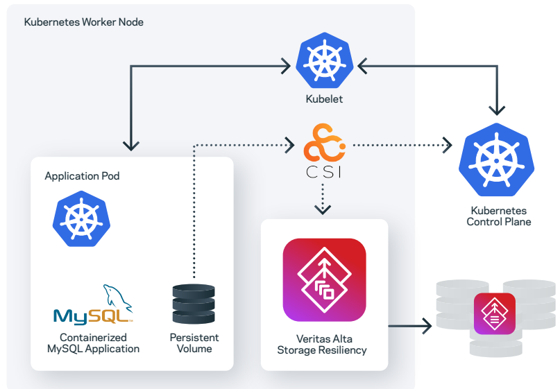
Figure 4. Veritas Alta Storage Resiliency CSI plug-in overview
