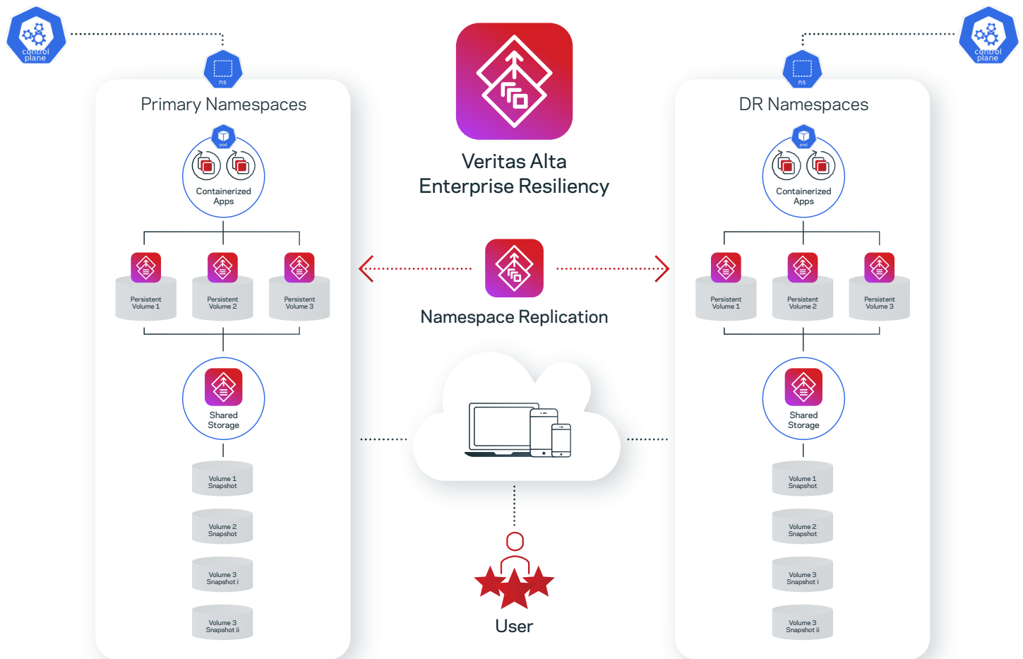
Figure 1. Veritas Alta Enterprise Resiliency and Veritas Alta Storage Resiliency for Kubernetes
