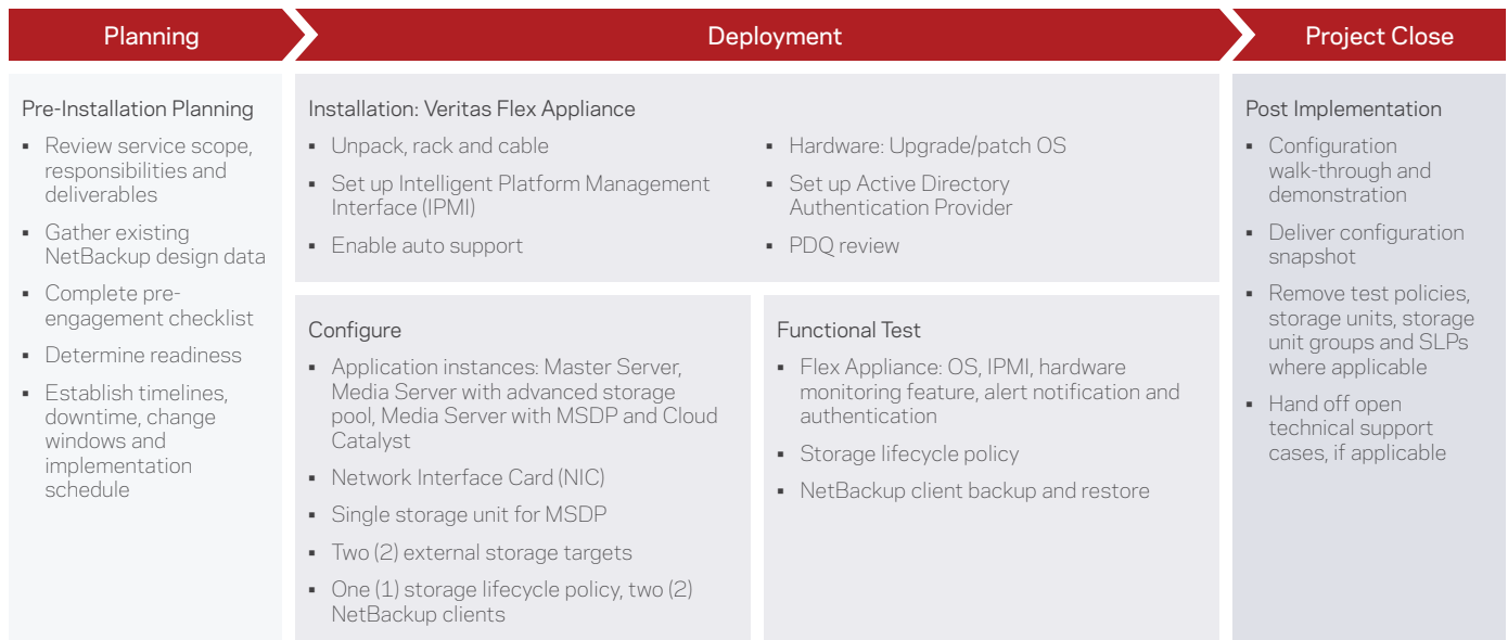
Figure 1. An overview of the Flex Appliance Implementation Service delivery process.
