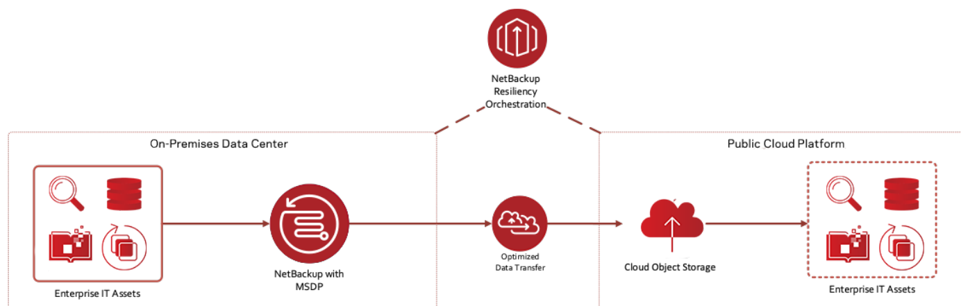
Figure 7. Automated cloud recovery using NetBackup images.
