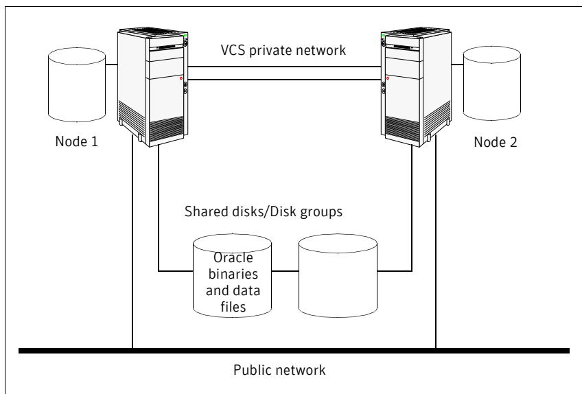
Figure 1-1 Oracle binaries and data on shared disks
