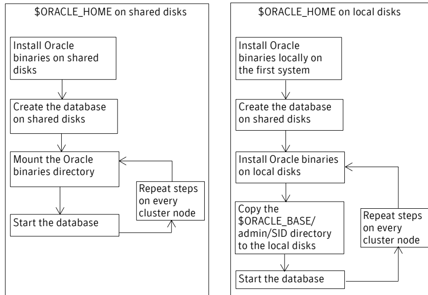
Figure 2-3 Comparison of the installation flow
