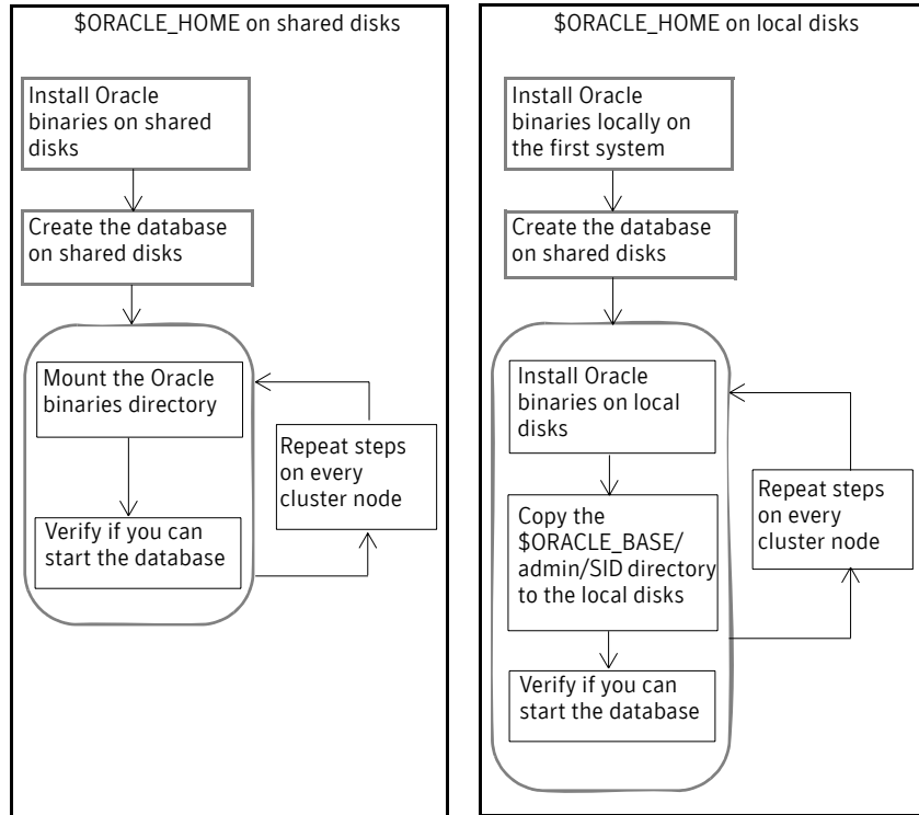
Figure 2-3 Comparison of the installation flow
