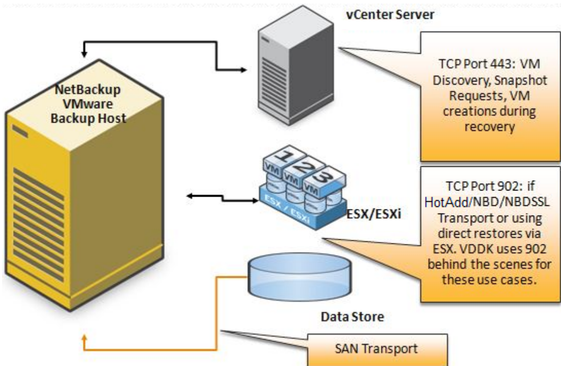
Figure 3-3 Ports VMware
