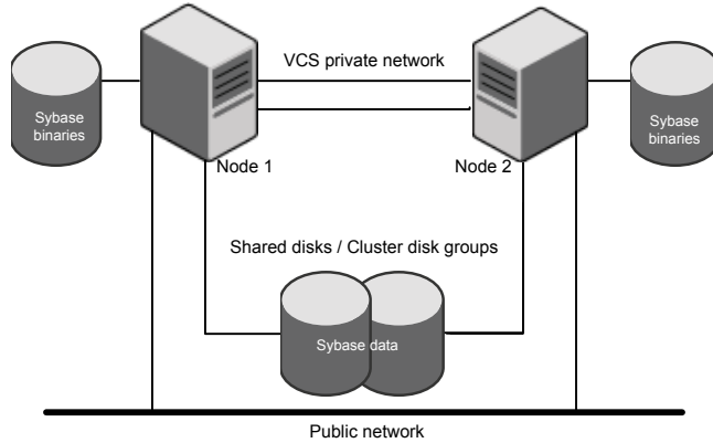
Figure 1-2 Binaries on local disk and Sybase data on shared disks
