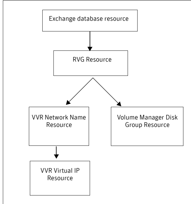
Figure 8-1 Dependency graph for Exchange Server
