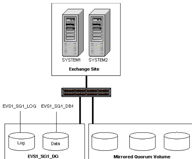
Figure 5-1 SFW disk groups and volumes for Exchange clustered mailbox server EVS1 in Microsoft clustering setup
