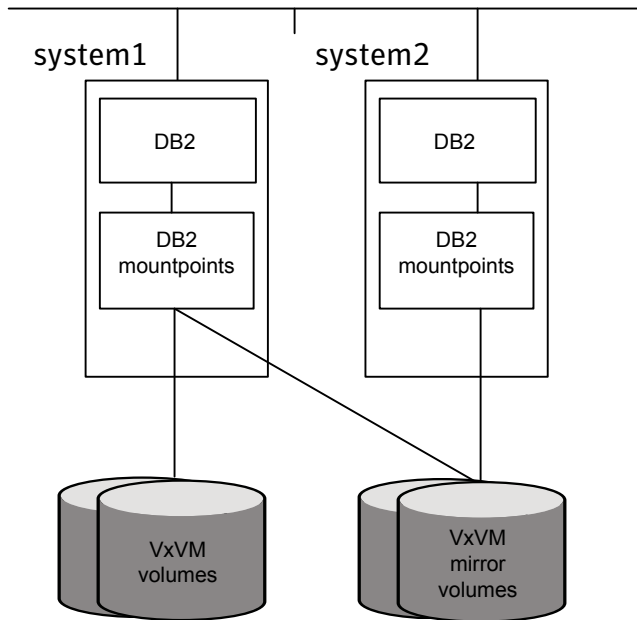
Figure 2-2 DB2 on a single system with off-host setup in Storage Foundation environment
