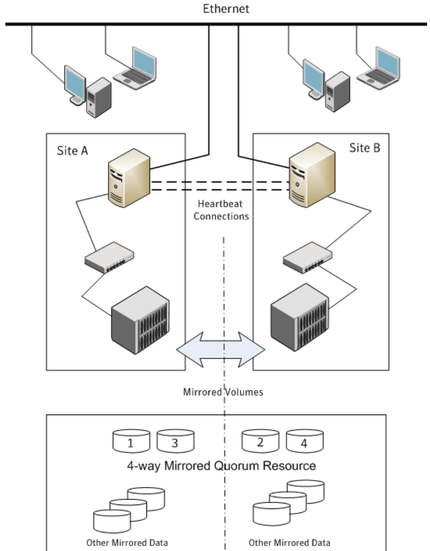
Figure 3-2 Typical campus clustering configuration
