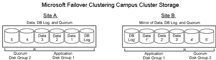
Figure 5-2 SFW disk groups and volumes for in a Microsoft campus cluster
