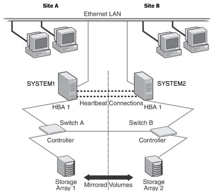
Figure 1-2 Campus cluster configuration example
