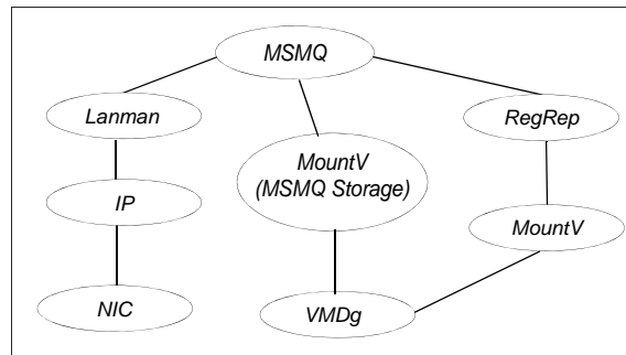
Figure 6-3 MSMQ agent dependency graph
