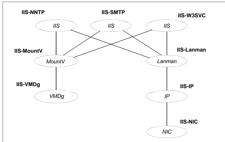
Figure 6-1 IIS service group dependency graph
