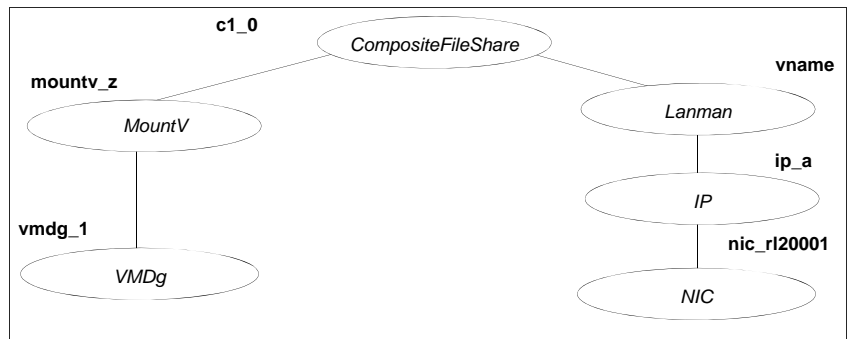
Figure 4-2 CompositeFileShare service group dependency graph
