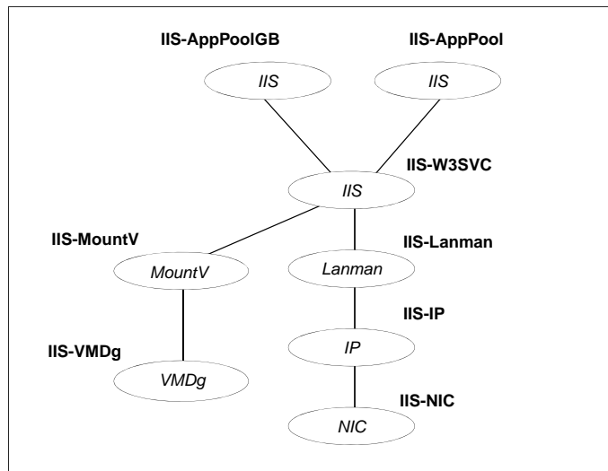
Figure 6-2 IIS service group dependency graph
