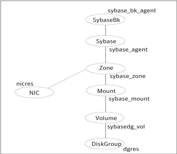
Figure B-2 Zone root on local disk
