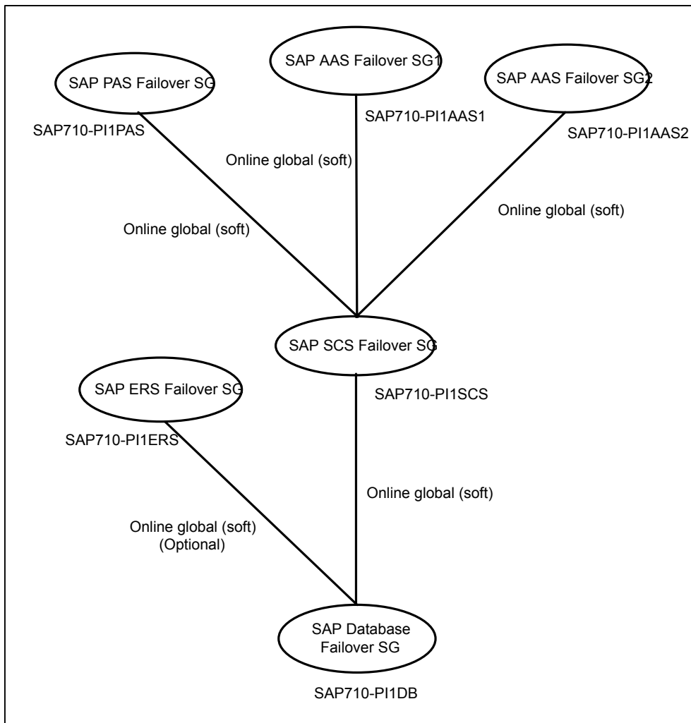
Figure A-5 Sample service group dependency
