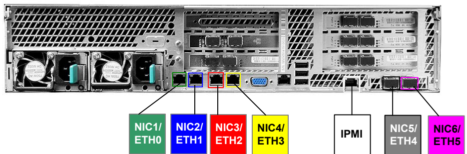
Figure 1-5 NetBackup 5330 Appliance compute node rear port colors
