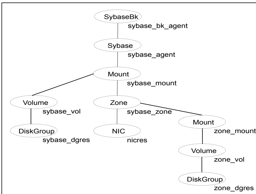
Figure B-3 Zone root on shared disk
