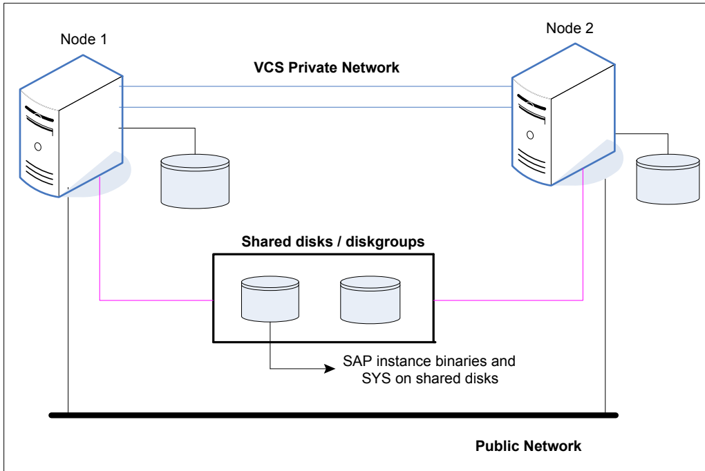
Figure 1-1 depicts a configuration where SAP Web Application Server instance binaries and SYS are installed completely on shared disks.
